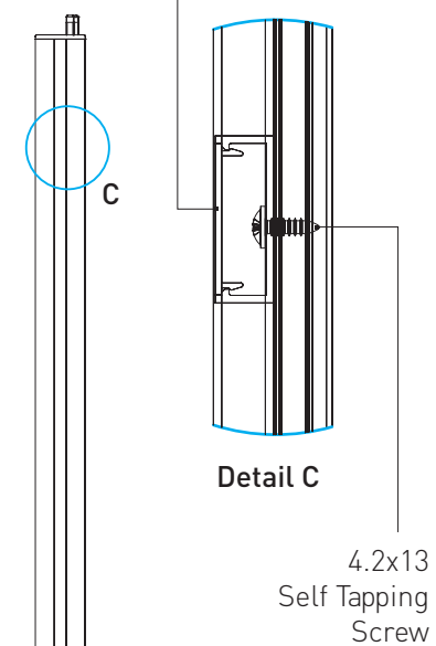
PR-9450 Cover for Horizontal Connector Profile
